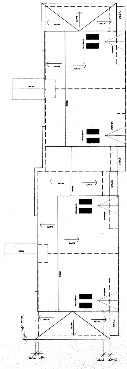
ROOF PLAN (BUILDING "B") 1/8" = 1'-0"
